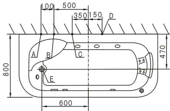
Horizontal dimensions
